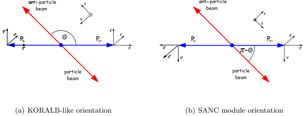
Figure 2: The relative orientation of reference frames for the spin states of \tau^+ , \tau^- and for hard processes as used in our interface (Fig. (a)) and in SANC module (Fig. (b)) are shown. In Fig (a) the axes x (not shown explicitly), x' and x'' are parallel to each other and point behind the picture, axis z is parallel to the direction of the anti-particle beam. In Fig (b) the axis z is parallel to the direction of the particle beam, the axis y' points behind the picture. Axes y (not shown explicitly) and y'' point toward the reader and are antiparallel to y' .
