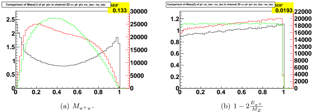
Figure 6: Longitudinal spin observables for the Z boson ( e^+e^- \rightarrow Z at 500 GeV). Distributions are shown for spin effects switched on (red), spin effects switched off (green), and their ratio (black). The plots are given in the default format of our example programs (included in the distribution tar ball). They are produced with the help of MC-TESTER [27]. Each plot is supplemented by an MC-TESTER defined titlebox and SDP parameter.
