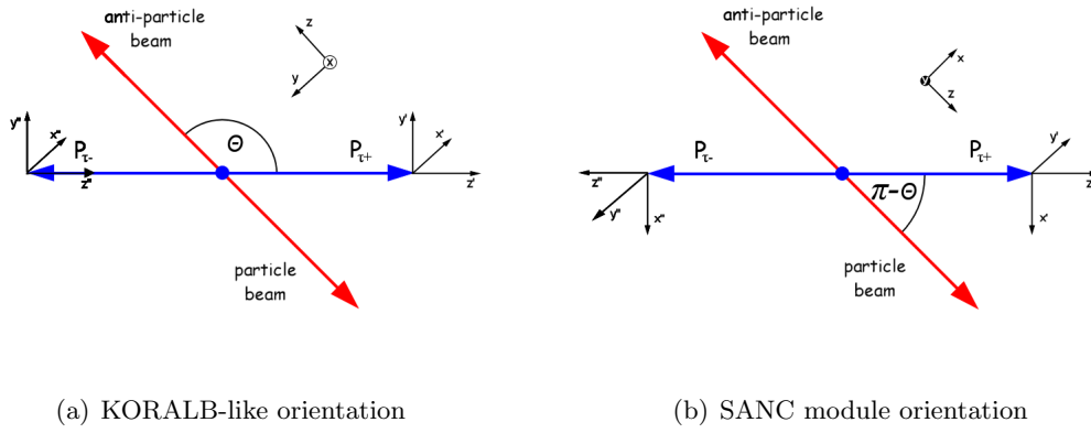
Figure 2: The relative orientation of reference frames for the spin states of \tau^+ , \tau^- and for hard processes as used in our interface (Fig. (a)) and in the SANC module (Fig. (b)) are shown. In Fig (a) the axes x (not shown explicitly), x' and x'' are parallel to each other and point behind the picture, axis z is parallel to the direction of the anti-particle beam. In Fig (b) the axis z is parallel to the direction of the particle beam, the axis y' points behind the picture. Axes y (not shown explicitly) and y'' point toward the reader and are antiparallel to y' .
