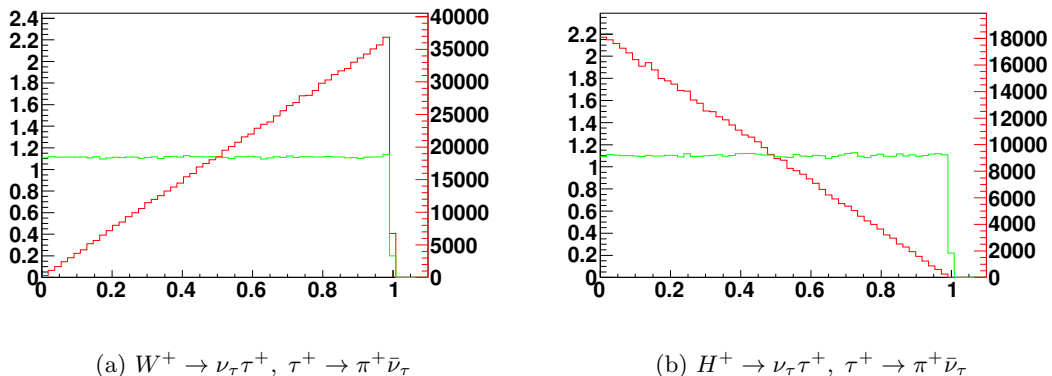
Figure 10: Pion energy spectrum in the rest frame of W (left hand side) and H^+ (right-hand side). Spin effects included (red line) and neglected (green line) are plotted. The variable 1 - 2 \frac{E_{\pi^+}}{M_{W^+}} or 1 - 2 \frac{E_{\pi^+}}{M_{H^+}} is used respectively.
