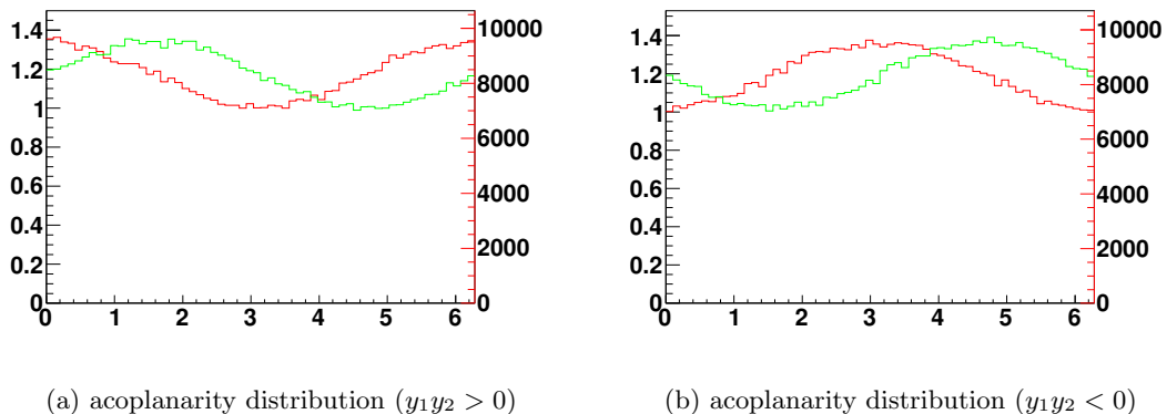
Figure 9: Transverse spin observables for the Higgs boson for \tau^\pm \rightarrow \pi^\pm \pi^0 \nu_\tau . Distributions are shown for scalar Higgs (red), scalar-pseudoscalar Higgs with mixing angle \frac{\pi}{4} (green). For the definition of angles see Section 6.2.
