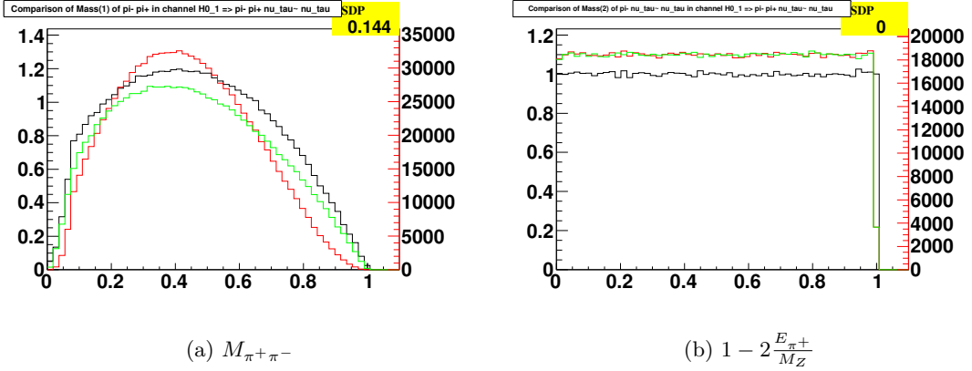
Figure 7: Longitudinal spin observables for the H boson for \tau^\pm \rightarrow \pi^\pm \nu_\tau . Distributions are shown for spin effects switched on (red), spin effects switched off (green), and their ratio (black). The plots are given in the default format of our example programs (included in the distribution tar ball). They are produced with the help of MC-TESTER [27]. Each plot is supplemented by an MC-TESTER defined titlebox and SDP parameter.
