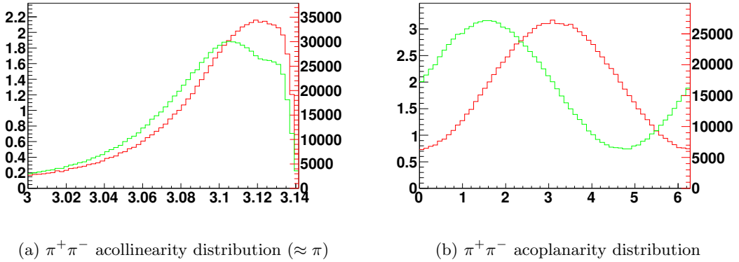
Figure 8: Transverse spin observables for the Higgs boson for \tau^\pm \rightarrow \pi^\pm \nu_\tau . Distributions are shown for scalar Higgs (red), scalar-pseudoscalar Higgs with mixing angle \frac{\pi}{4} . For the definition of angles see Section 6.2.
