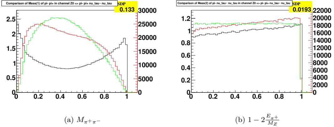
Figure 6: Longitudinal spin observables for the Z boson ( e^+e^- \rightarrow Z at 500 GeV). Distributions are shown for spin effects switched on (red), spin effects switched off (green), and their ratio (black). The plots are given in the default format of our example programs (included in the distribution tar ball). They are produced with the help of MC-TESTER [27]. Each plot is supplemented by an MC-TESTER defined titlebox and SDP parameter.
